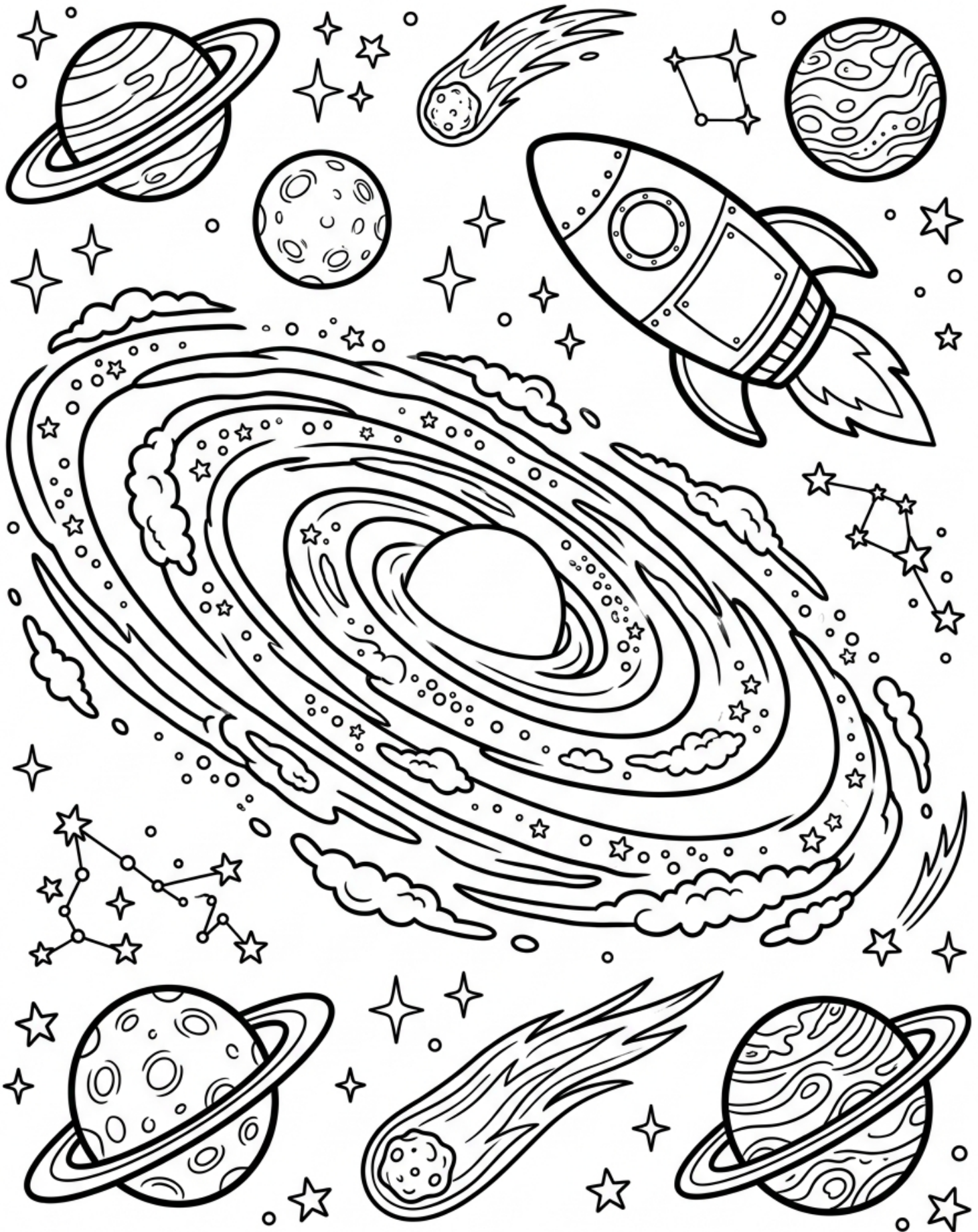
Galaxy Spiral
