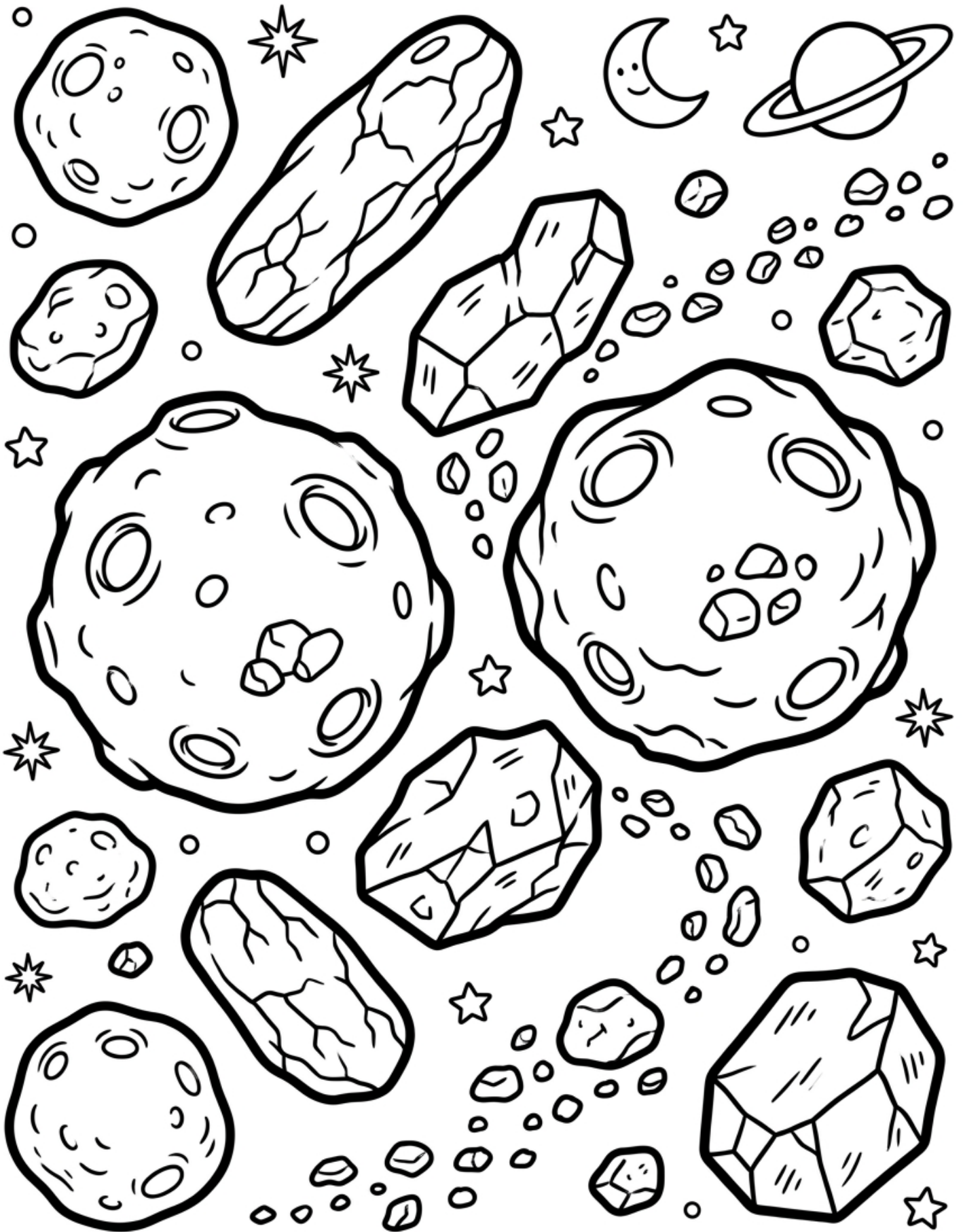
Asteroid Belt
