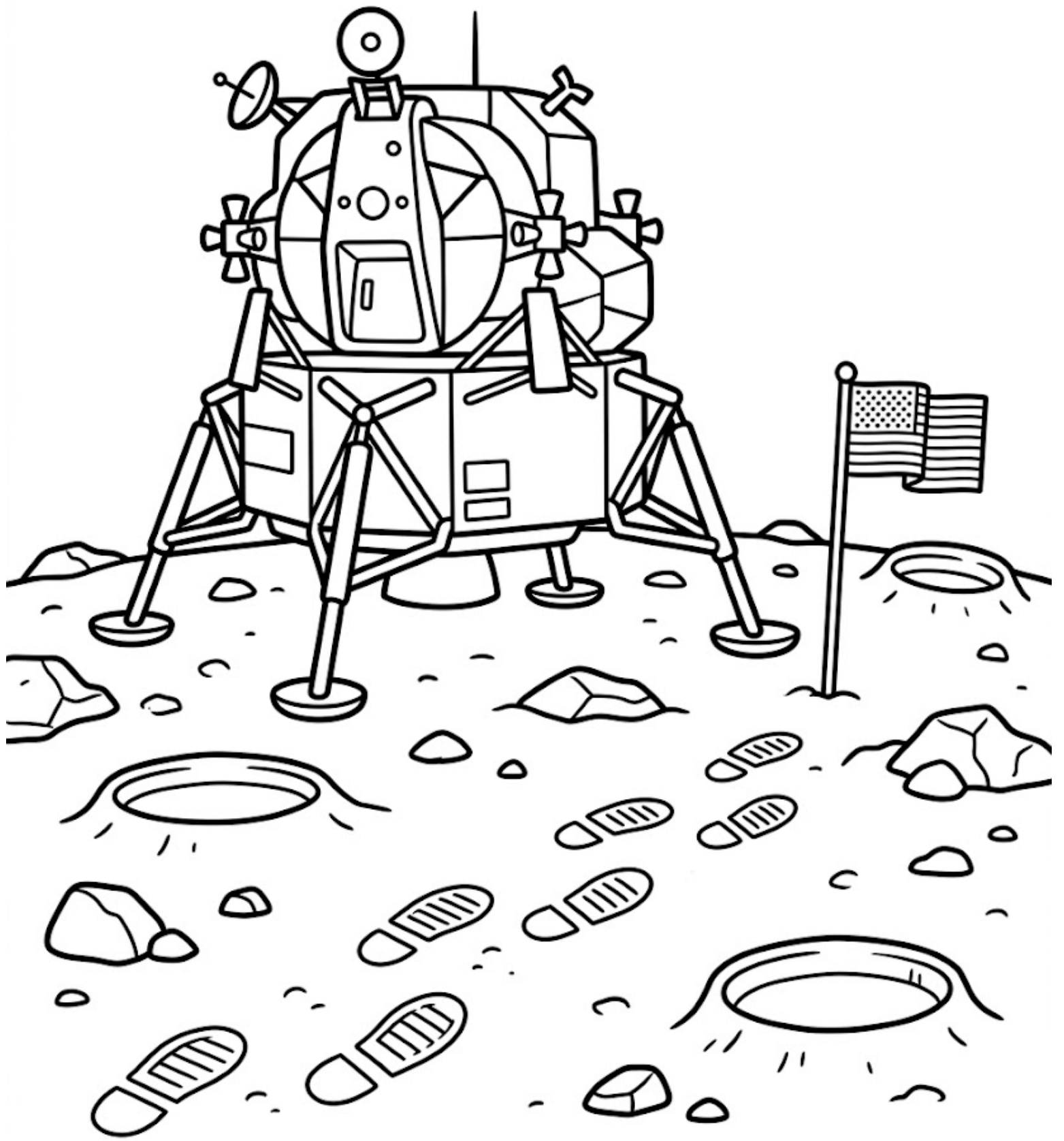
Moon Landing
