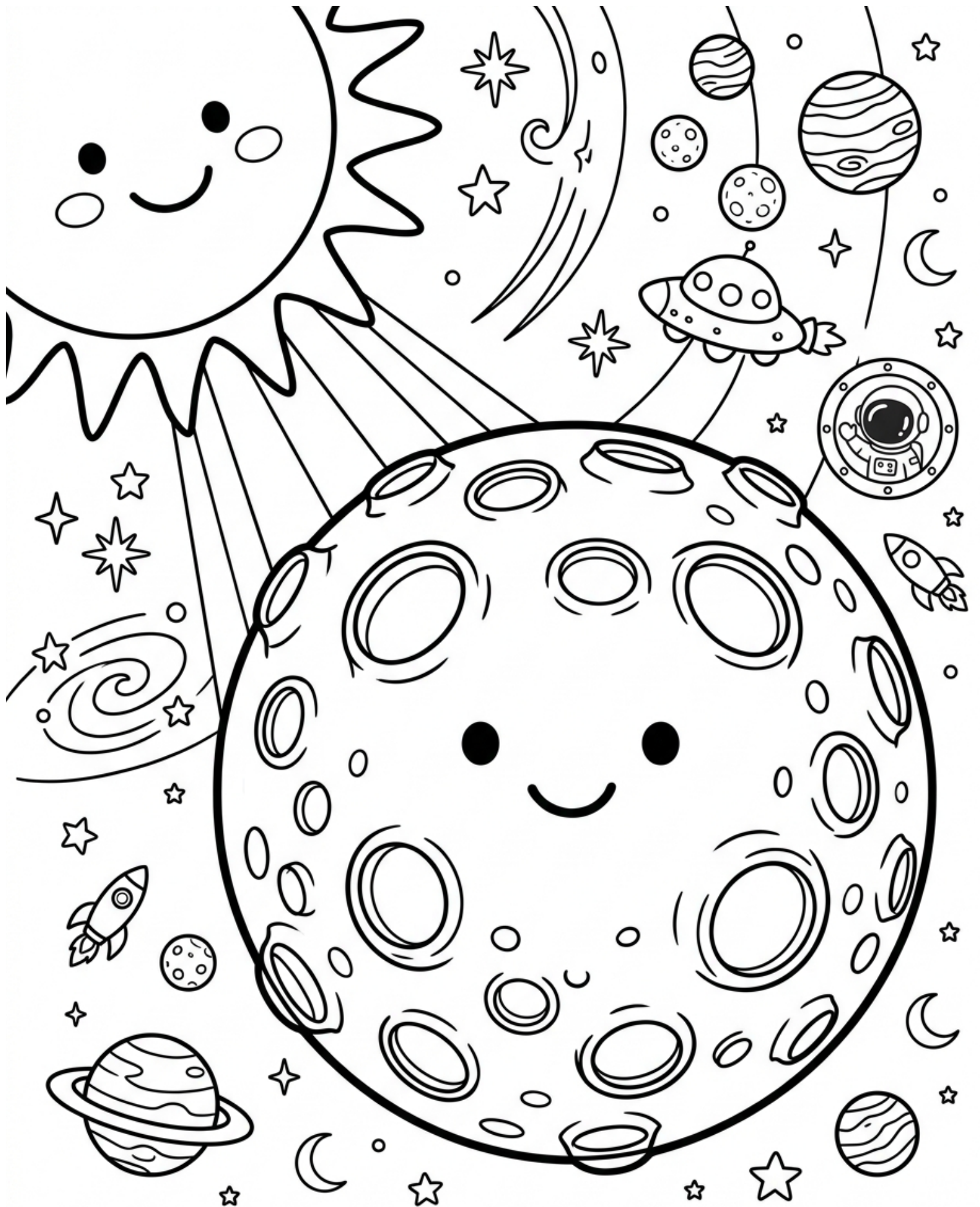
Mercury Craters
