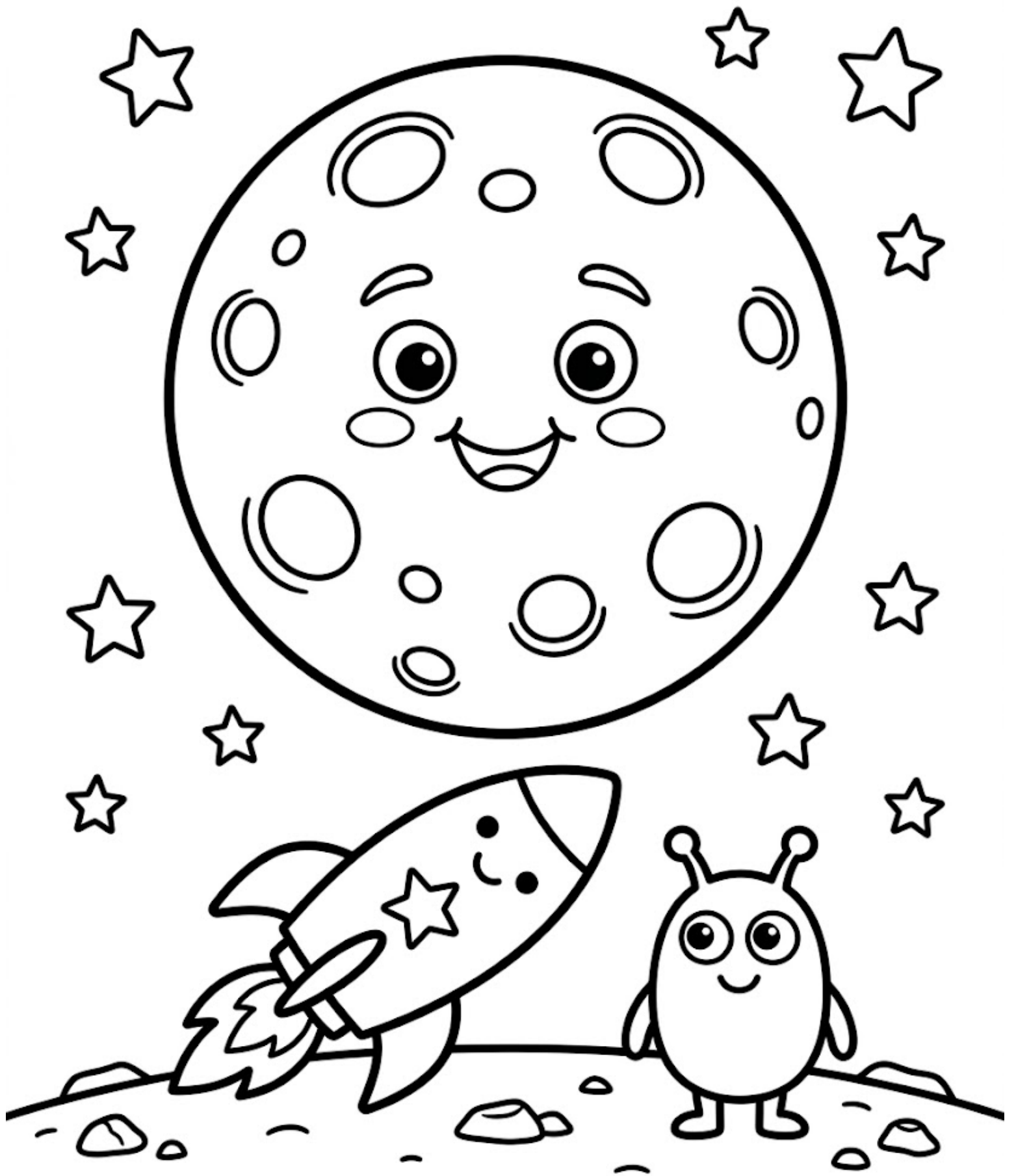
Round Moon
